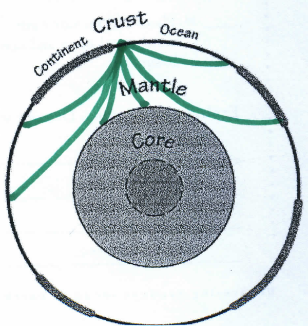
S-wave
