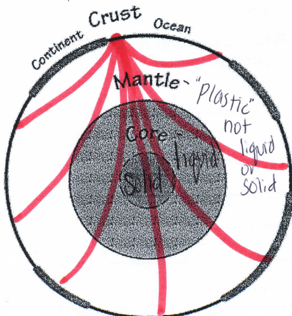
P-wave
